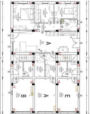
piano piano terra - SX
